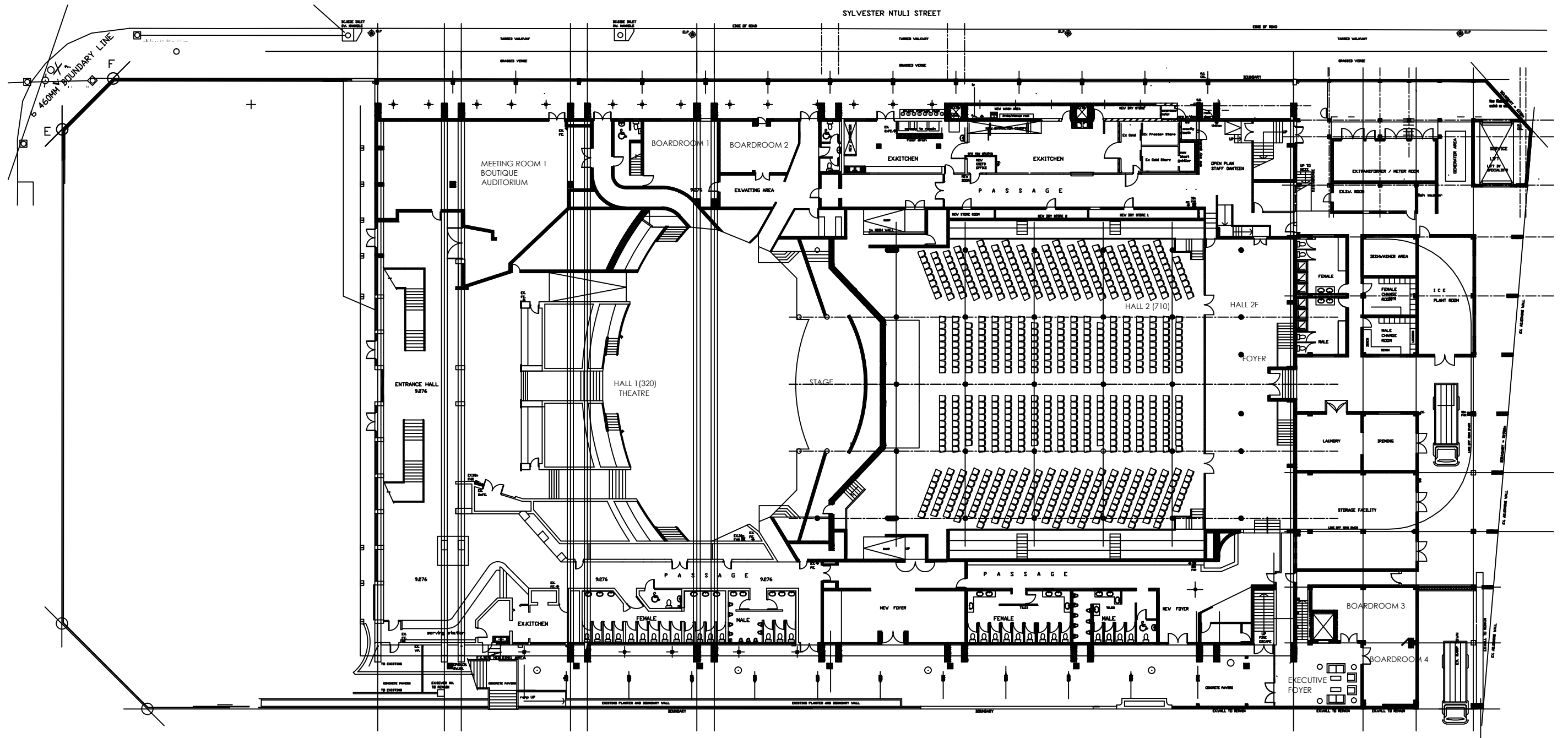
LOWER GROUND STOREY
